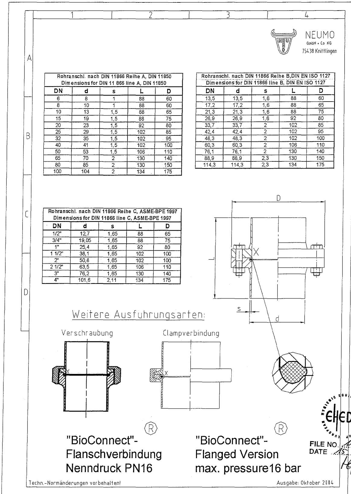
Fig.: pipe connection, type BioConnect®
